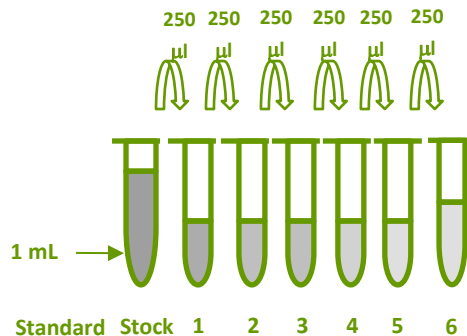
Concentration 400 200 100 50 25 12.5 6.25 pg/ml
